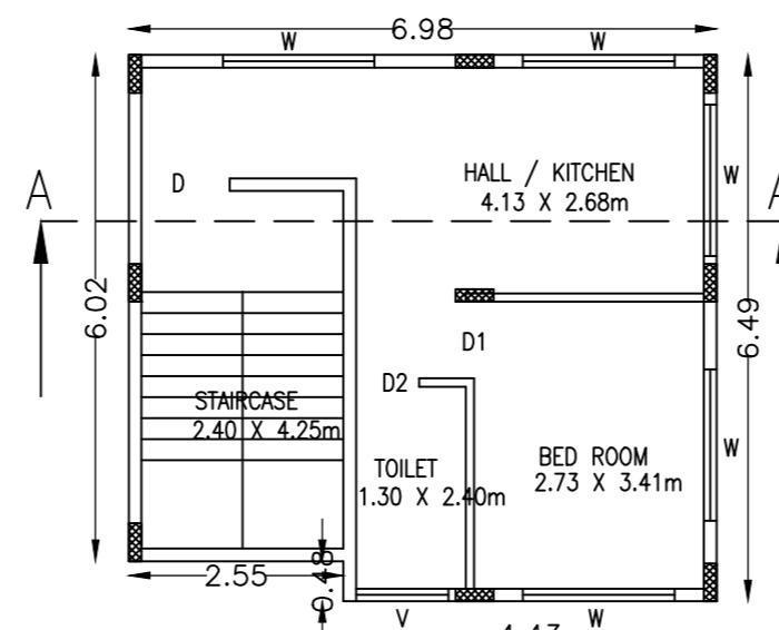
PROPOSED TYPICAL FLOOR PLAN FOR FIRST AND SECOND FLOOR PLAN
